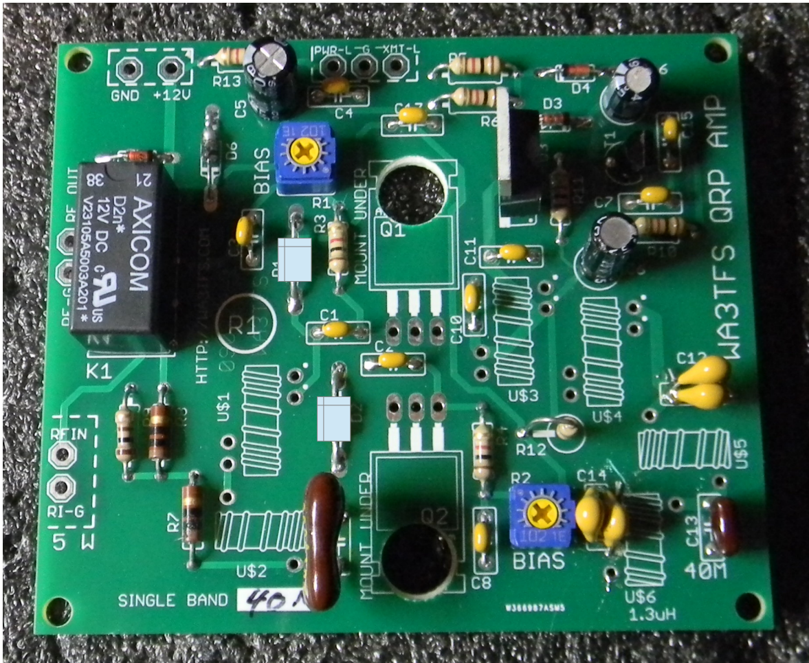
FIGURE 7 Install the capacitors in the tuned sections of the circuit. In the photo, I have combined some capacitors to match the required values at C12 and C14, but just install the components detailed on the parts list. Capacitors installed at this stage are C9, C12, C13, and C14.
