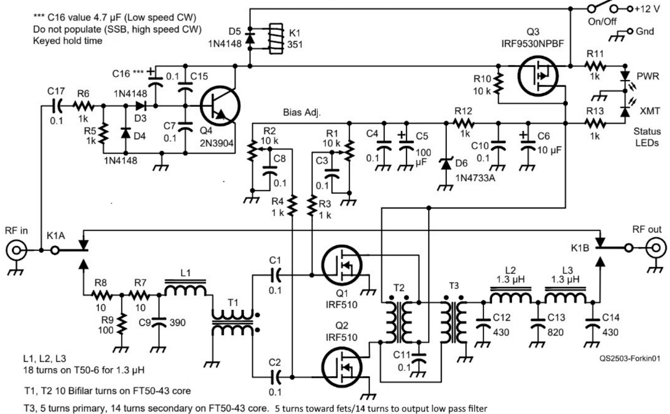
SCHMATIC AS PUBLISHED IN QST MAGAZINE
