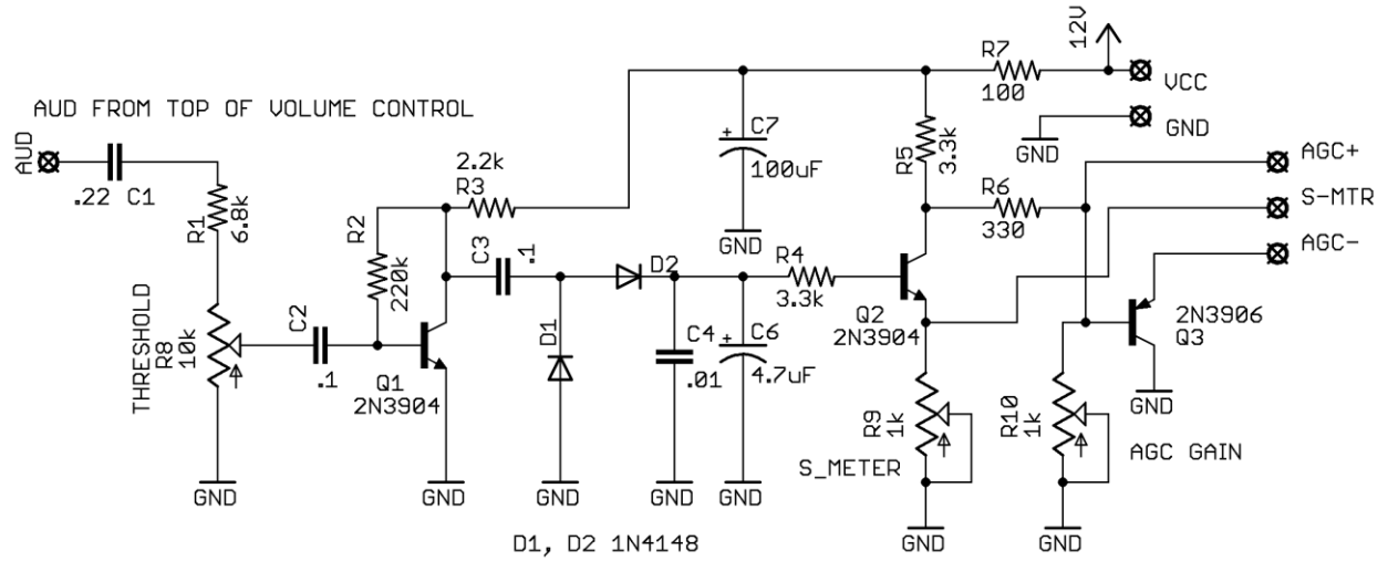
WA3TFS AGC CIRCUIT FOR THE SIONGLE BAND RECEIVER
